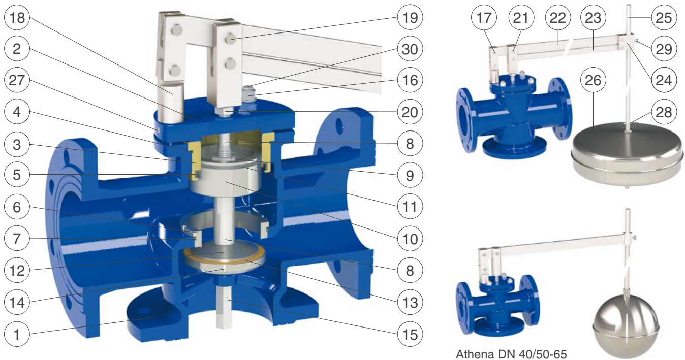
Athena DN 40/50-65
